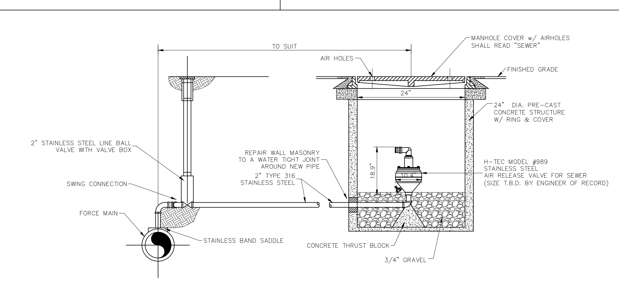
5 TYPICAL AIR AND/OR VACUUM VALVES N.T.S.
