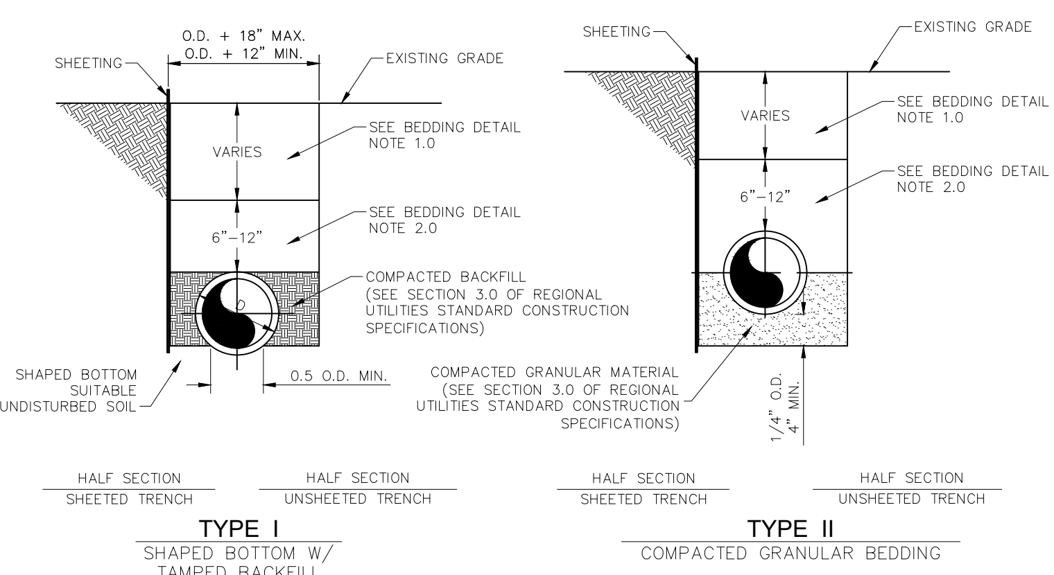
3 TYPICAL BEDDING DETAIL N.T.S.
