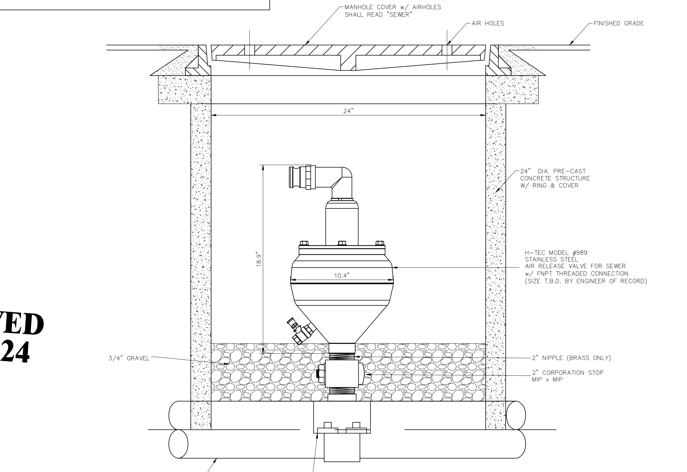
6 TYPICAL PRESSURE SEWER AIR RELEASE MANHOLE N.T.S.
